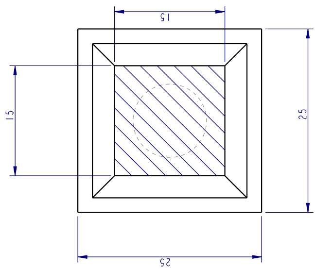
SECTION 2-2
